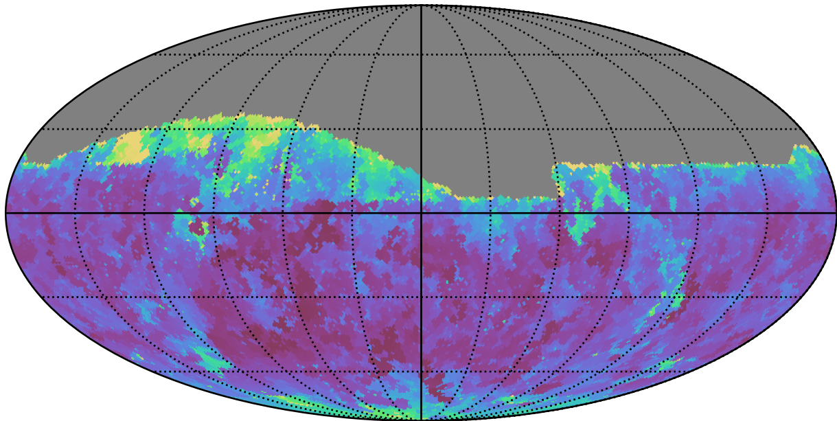
ddf_loaded_half_fl4_v3.4_10yrs Yr 1 z band: Min seeingEff
