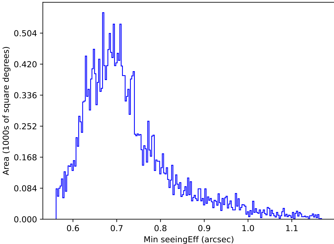
ddf_loaded_half_fl4_v3.4_10yrs Yr 1 z band: Min seeingEff
