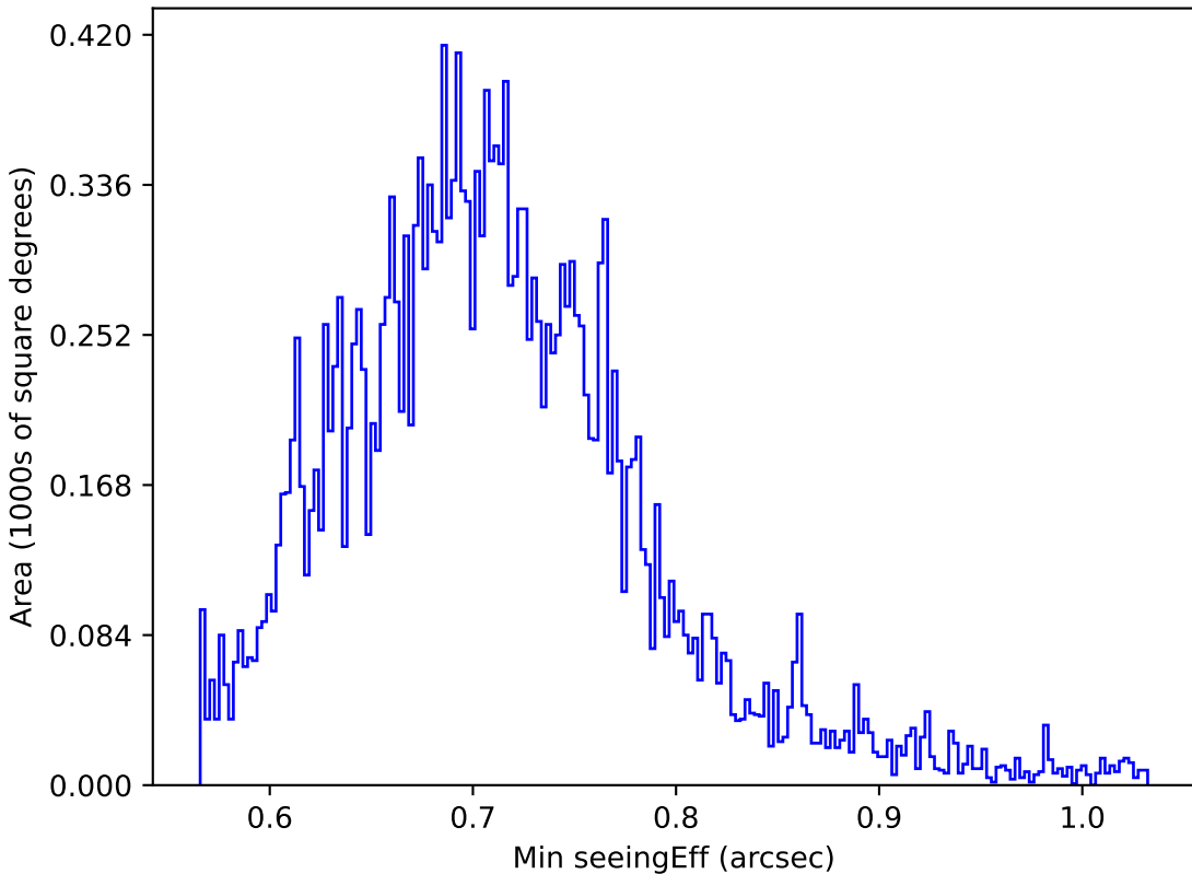
ddf_loaded_half_fl4_v3.4_10yrs Yr 1 y band: Min seeingEff
