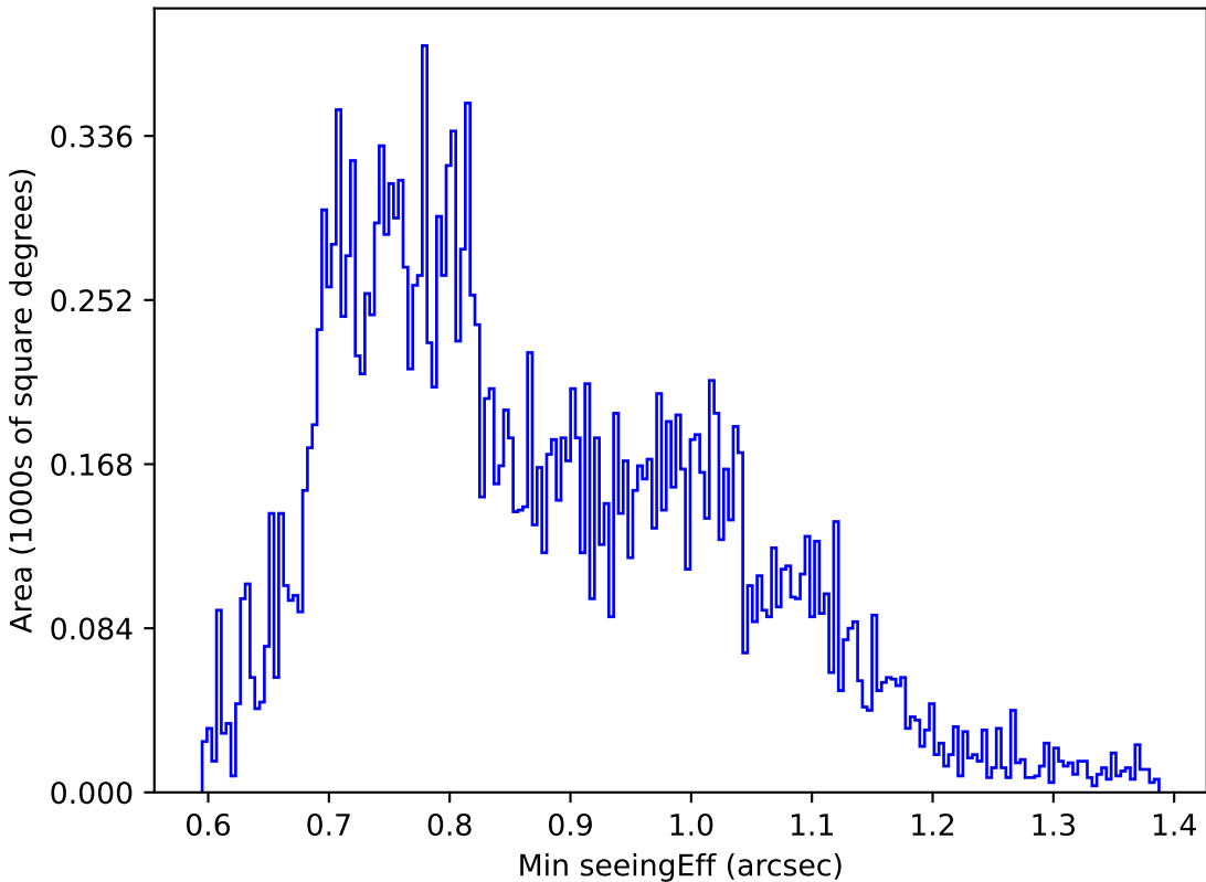
ddf_loaded_half_fl4_v3.4_10yrs Yr 1 u band: Min seeingEff
