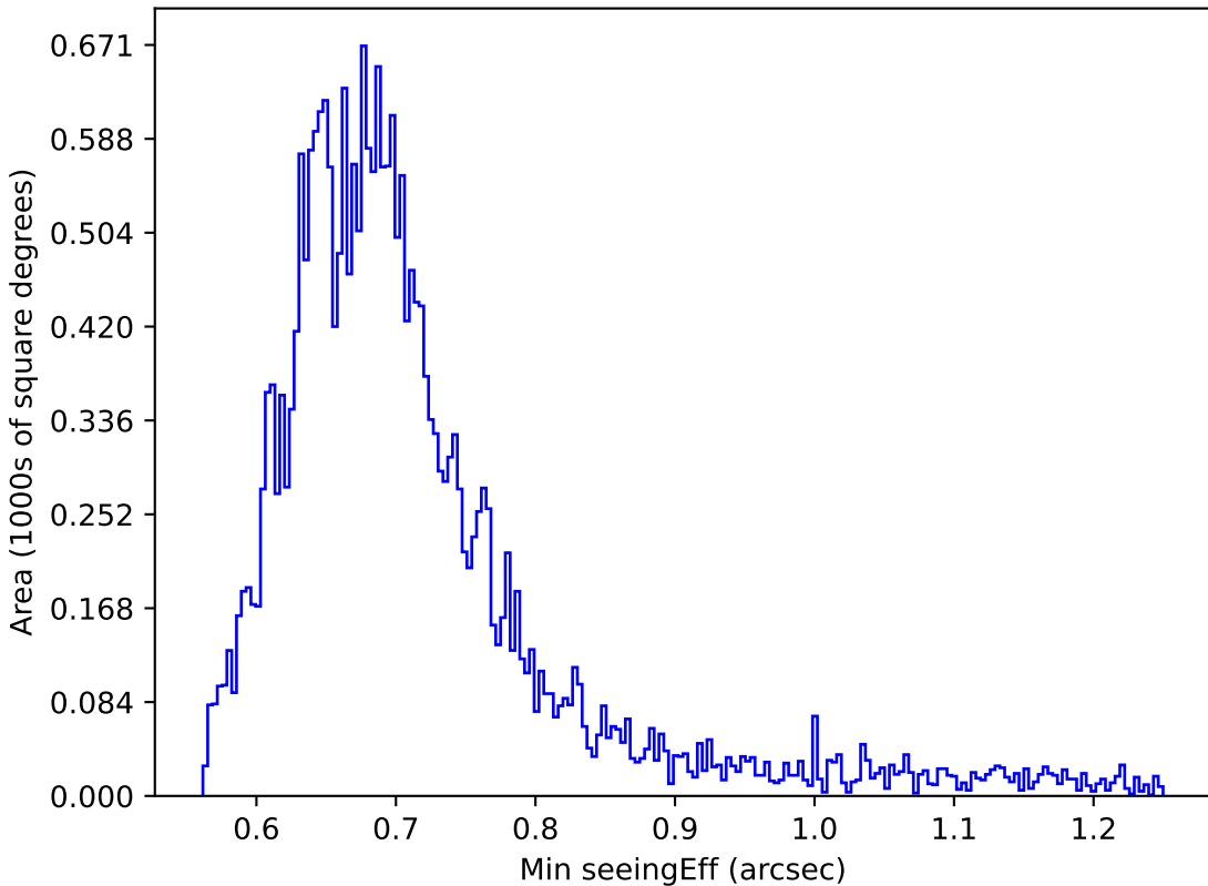
ddf_loaded_half_fl4_v3.4_10yrs Yr 1 r band: Min seeingEff
