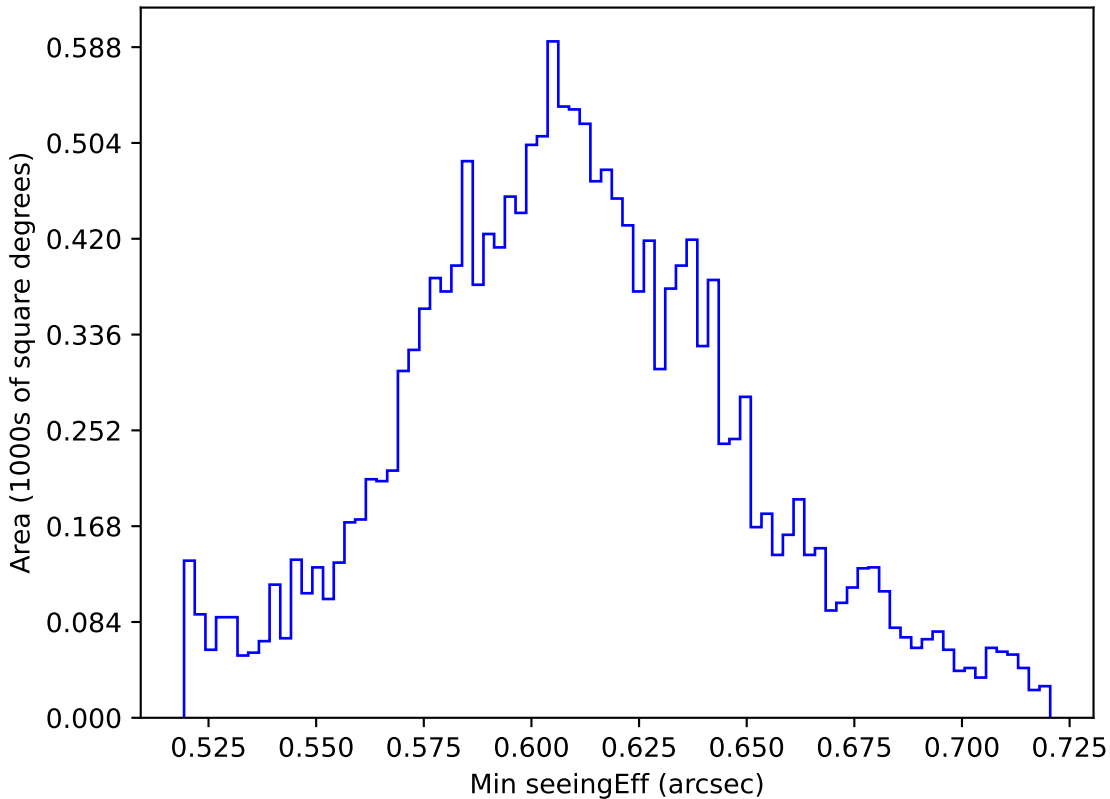
ddf_loaded_half_fl4_v3.4_10yrs WFD z band: Min seeingEff
