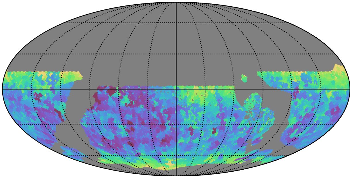
ddf_loaded_half_fl4_v3.4_10yrs WFD y band: Min seeingEff
