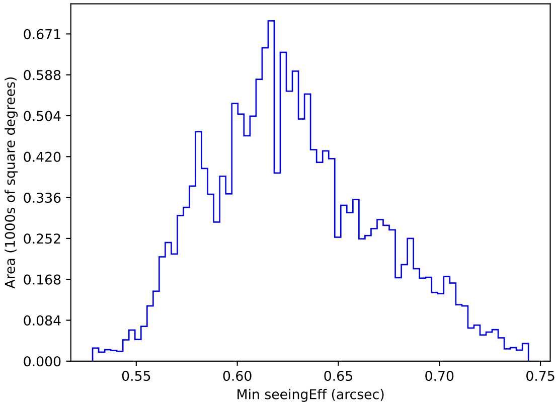
ddf_loaded_half_fl4_v3.4_10yrs WFD y band: Min seeingEff
