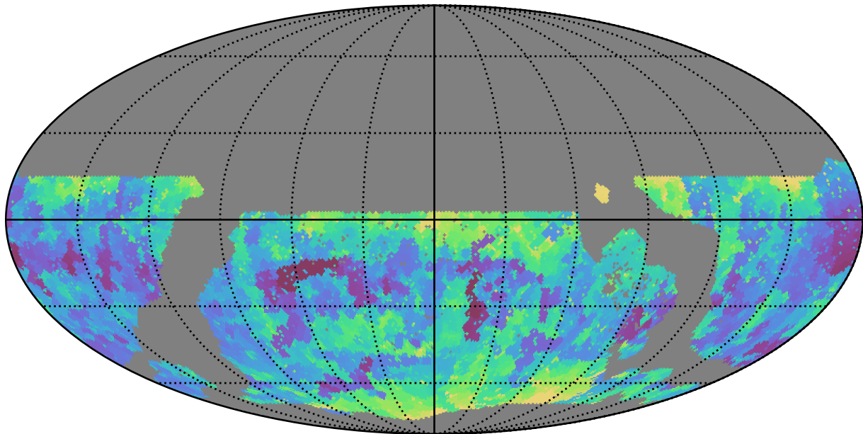
ddf_loaded_half_fl4_v3.4_10yrs WFD u band: Min seeingEff
