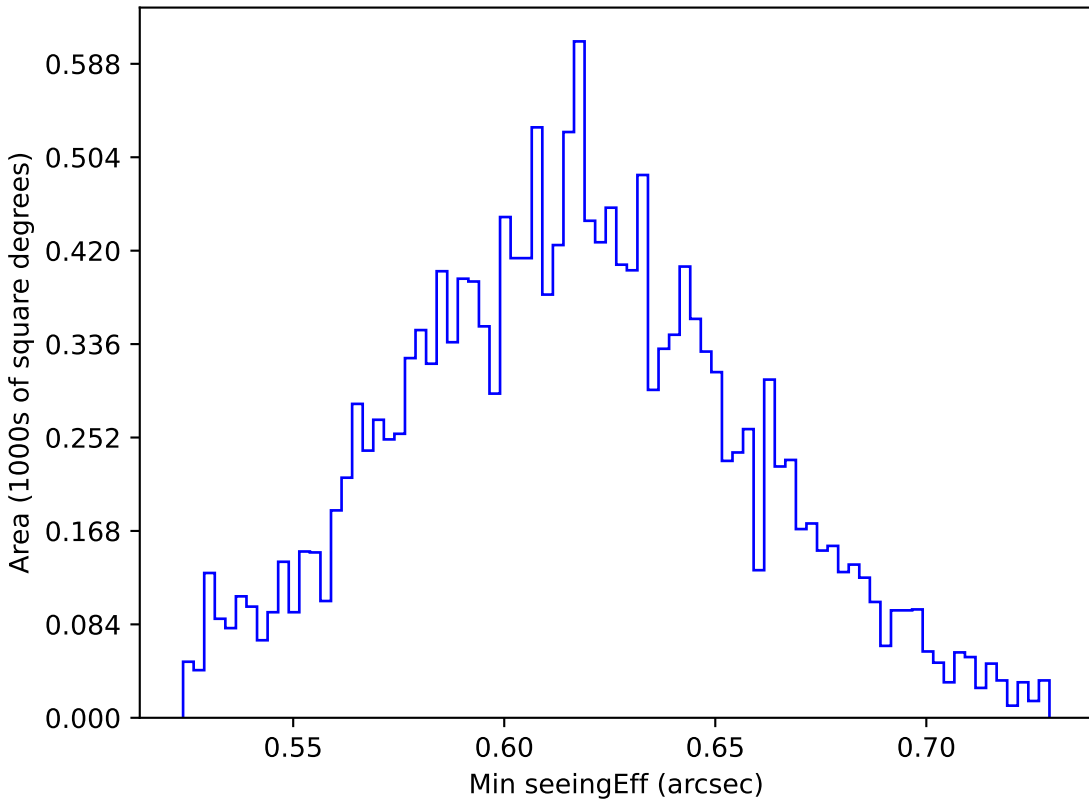
ddf_loaded_half_fl4_v3.4_10yrs WFD r band: Min seeingEff
