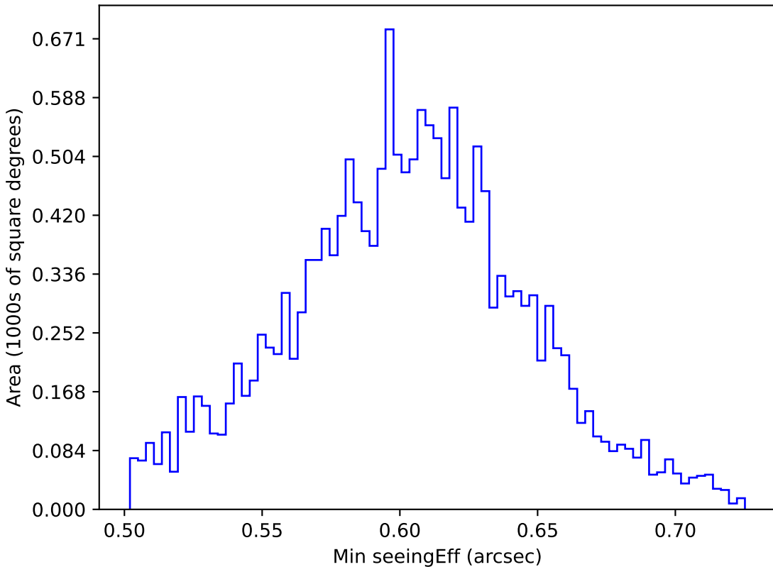
ddf_loaded_half_fl4_v3.4_10yrs WFD i band: Min seeingEff
