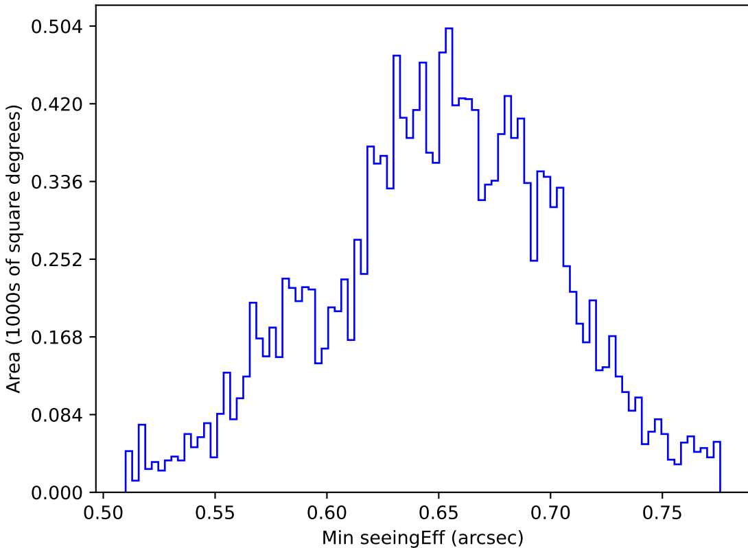
ddf_loaded_half_fl4_v3.4_10yrs WFD g band: Min seeingEff
