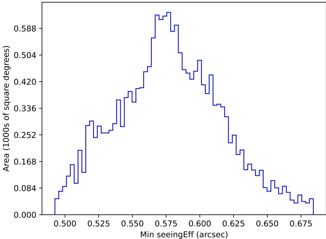
ddf_loaded_half_fl4_v3.4_10yrs WFD all bands: Min seeingEff
