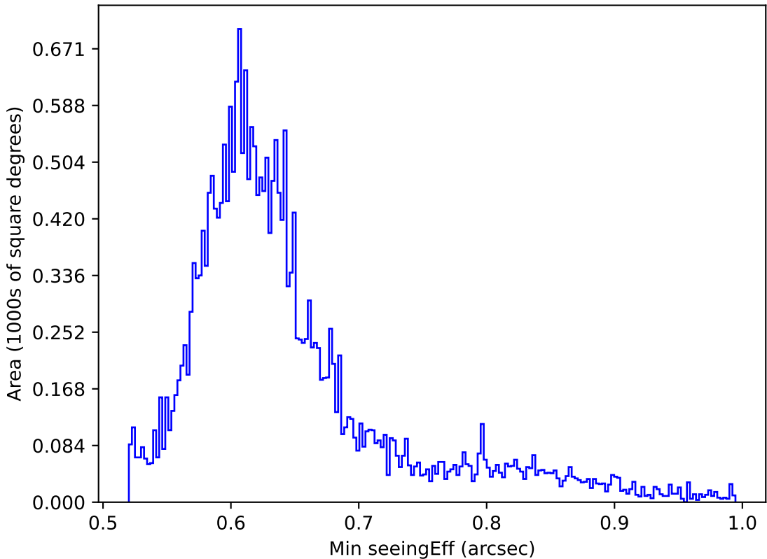
ddf_loaded_half_fl4_v3.4_10yrs All sky z band: Min seeingEff
