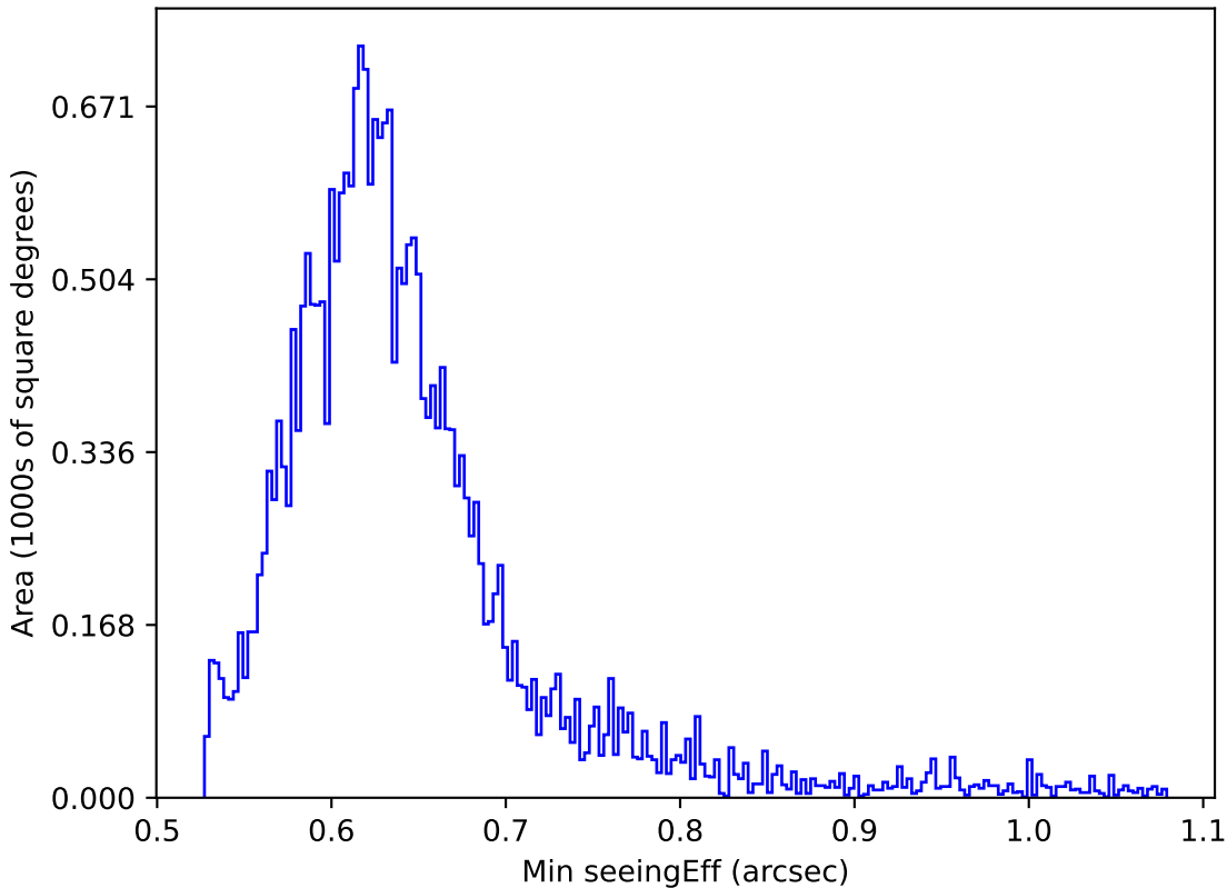
ddf_loaded_half_fl4_v3.4_10yrs All sky r band: Min seeingEff
