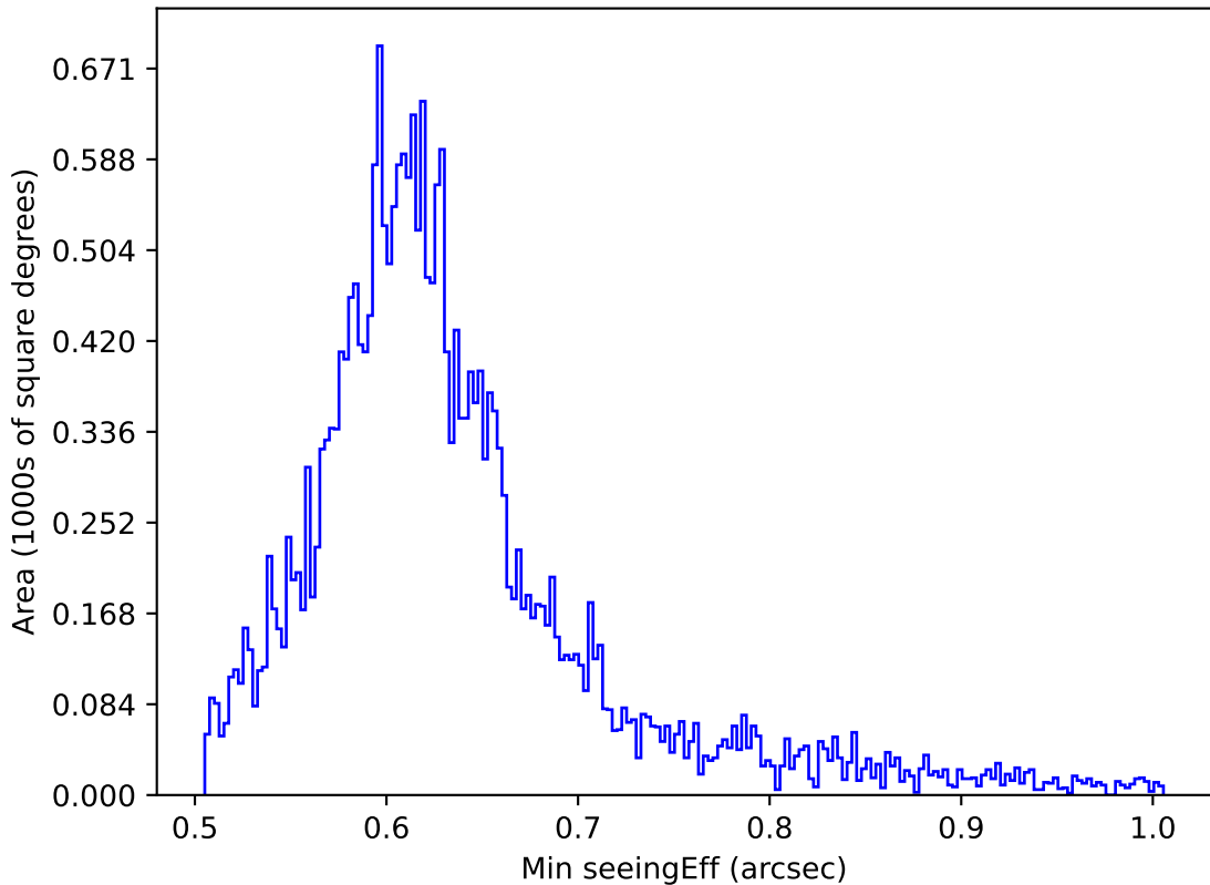
ddf_loaded_half_fl4_v3.4_10yrs All sky i band: Min seeingEff
