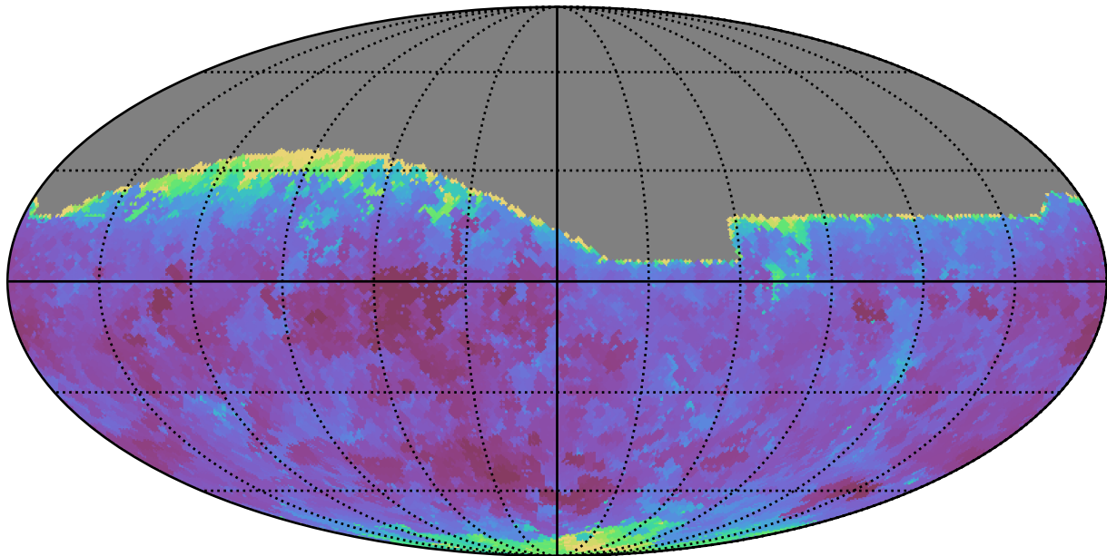
ddf_loaded_half_fl4_v3.4_10yrs All sky g band: Min seeingEff
