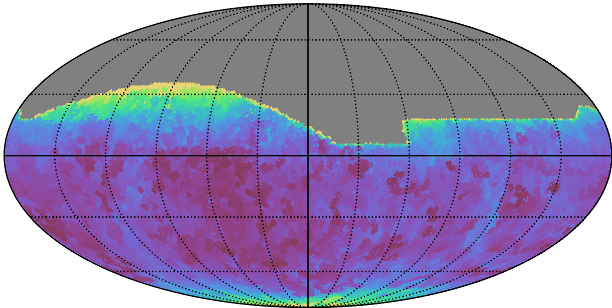
ddf_loaded_half_fl4_v3.4_10yrs All sky all bands: Min seeingEff
