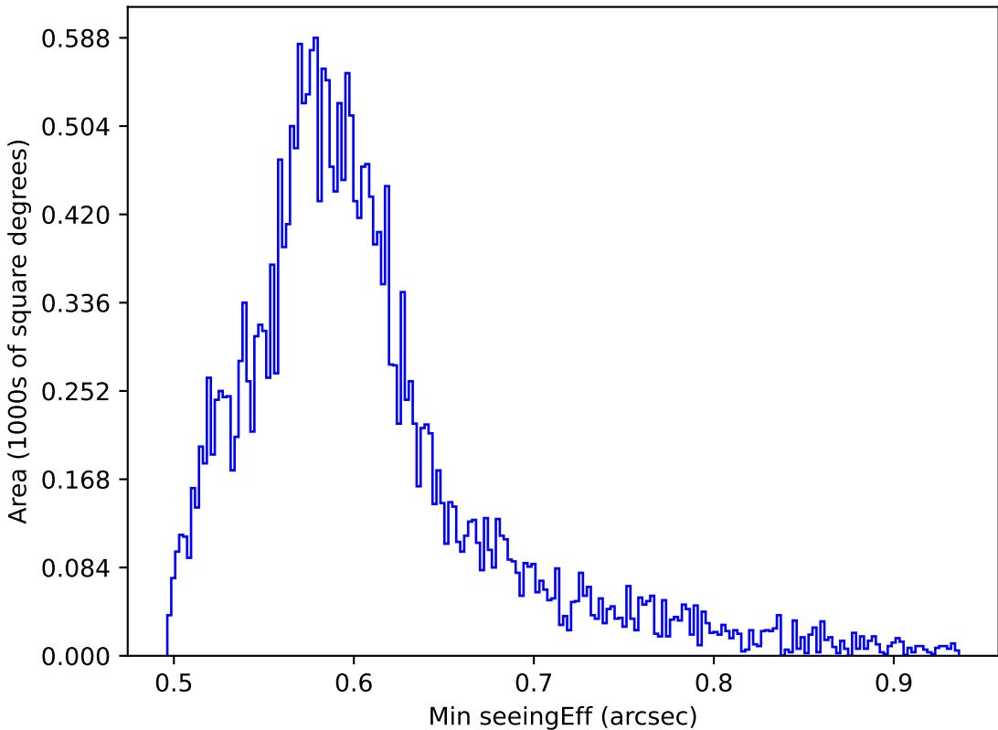
ddf_loaded_half_fl4_v3.4_10yrs All sky all bands: Min seeingEff
