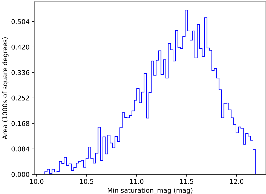
ddf_loaded_half_fl4_v3.4_10yrs WFD u band: Min saturation_mag
