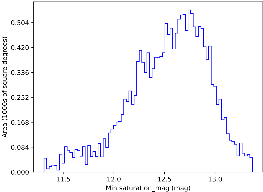
ddf_loaded_half_fl4_v3.4_10yrs WFD r band: Min saturation_mag
