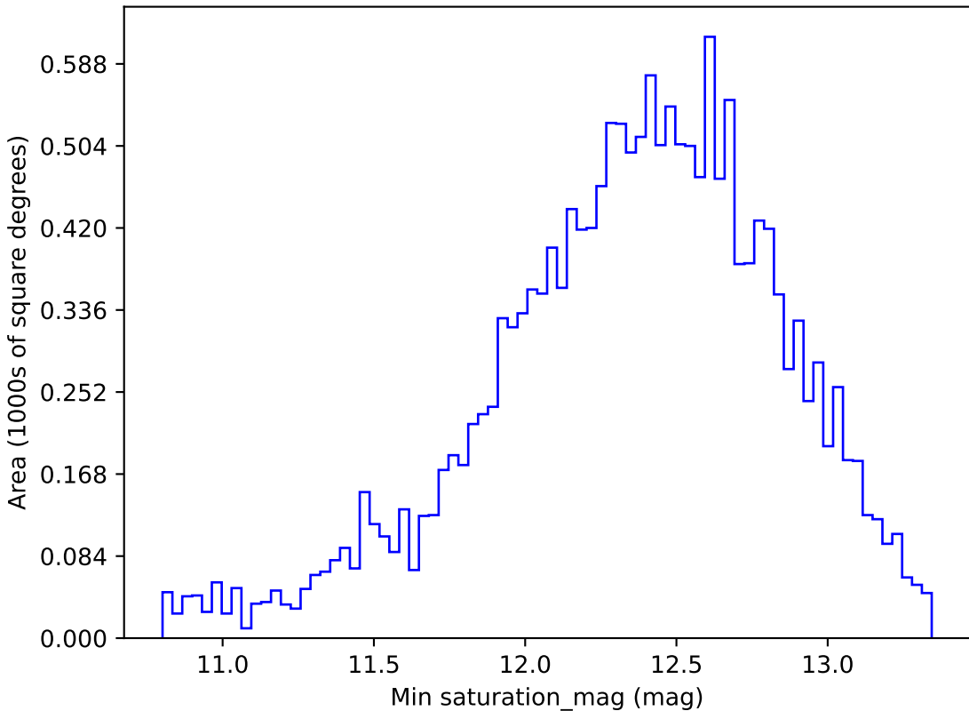
ddf_loaded_half_fl4_v3.4_10yrs WFD i band: Min saturation_mag
