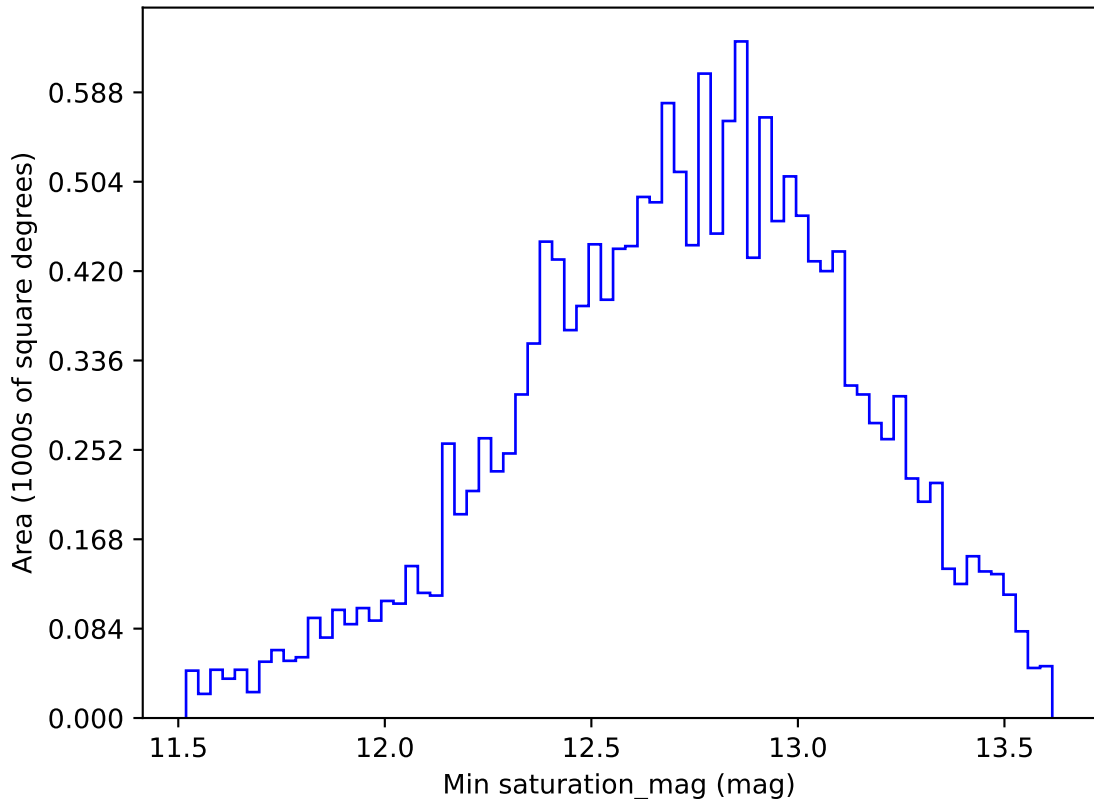
ddf_loaded_half_fl4_v3.4_10yrs WFD g band: Min saturation_mag
