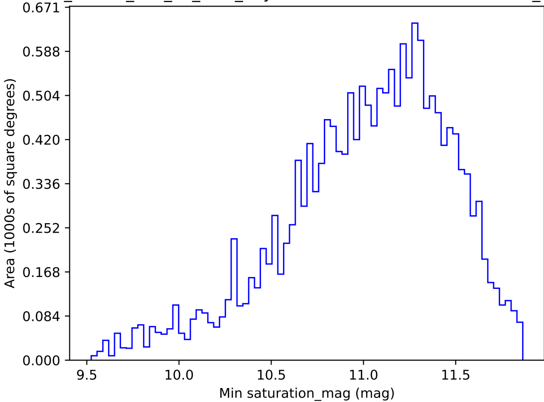
ddf_loaded_half_f14_v3.4_10yrs WFD all bands: Min saturation_mag
