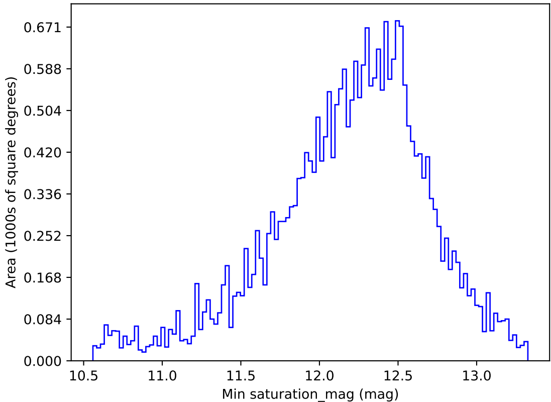
ddf_loaded_half_fl4_v3.4_10yrs All sky z band: Min saturation_mag
