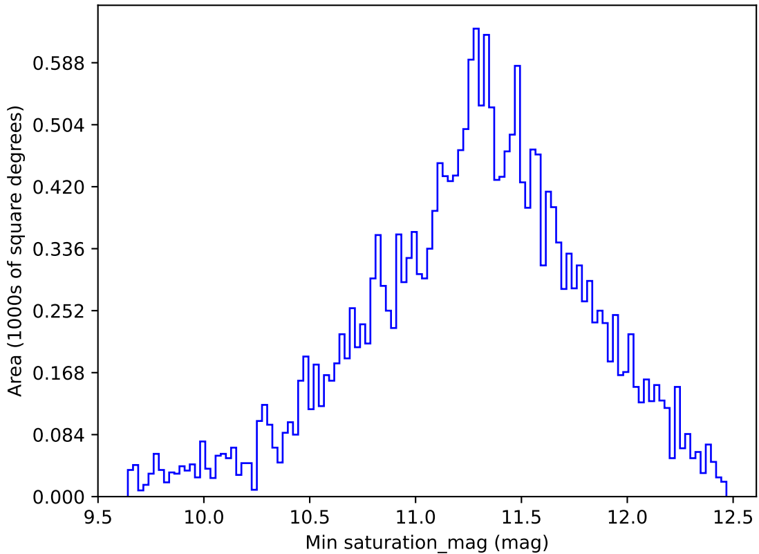
ddf_loaded_half_fl4_v3.4_10yrs All sky y band: Min saturation_mag
