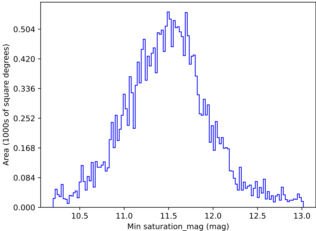
ddf_loaded_half_fl4_v3.4_10yrs All sky u band: Min saturation_mag
