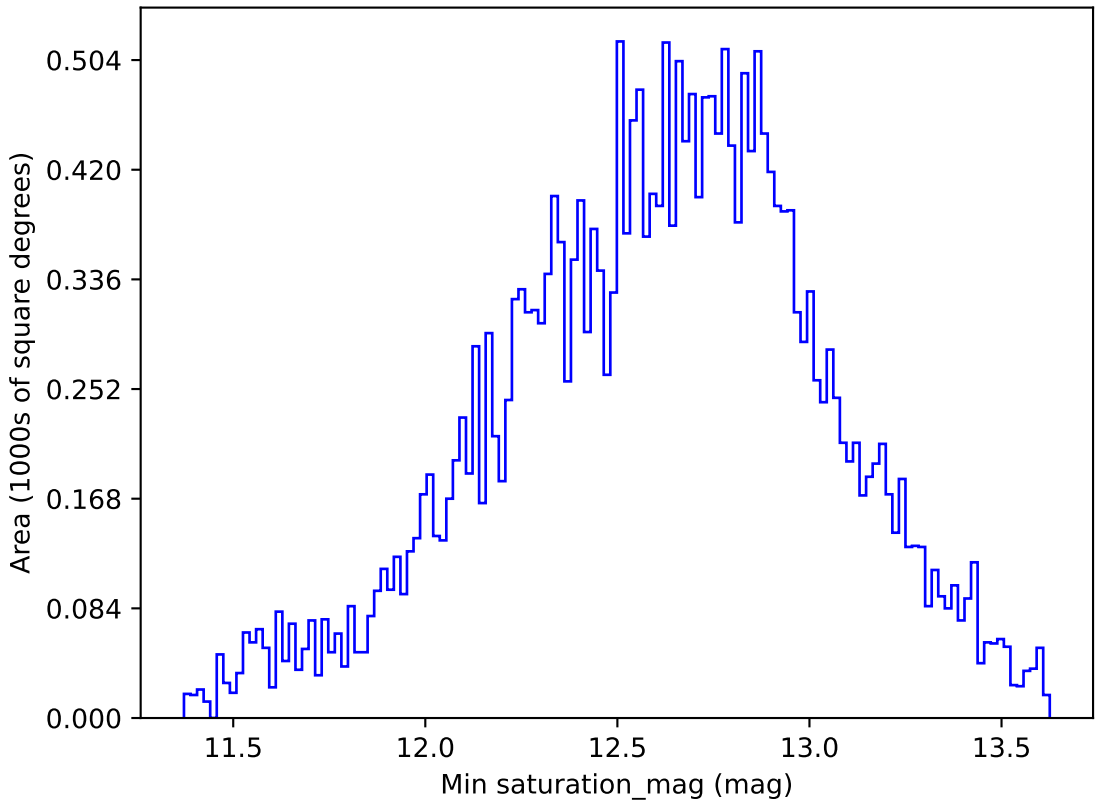
ddf_loaded_half_fl4_v3.4_10yrs All sky r band: Min saturation_mag
