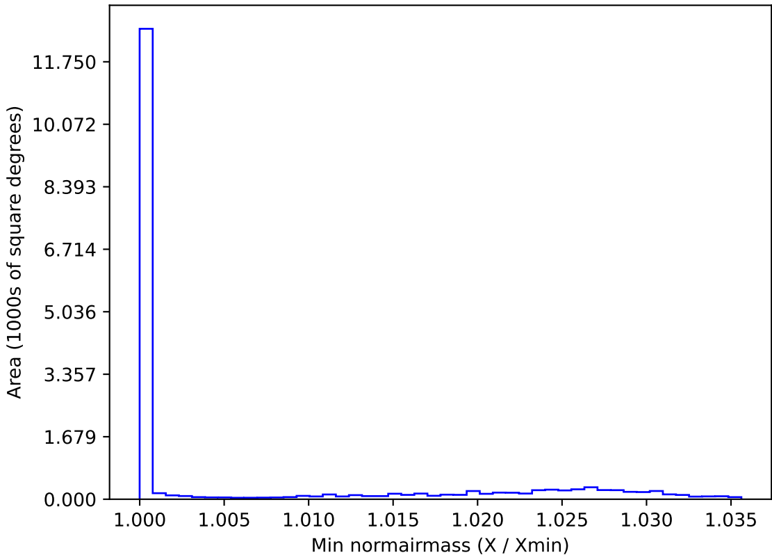
ddf_loaded_half_fl4_v3.4_10yrs WFD z band: Min normairmass
