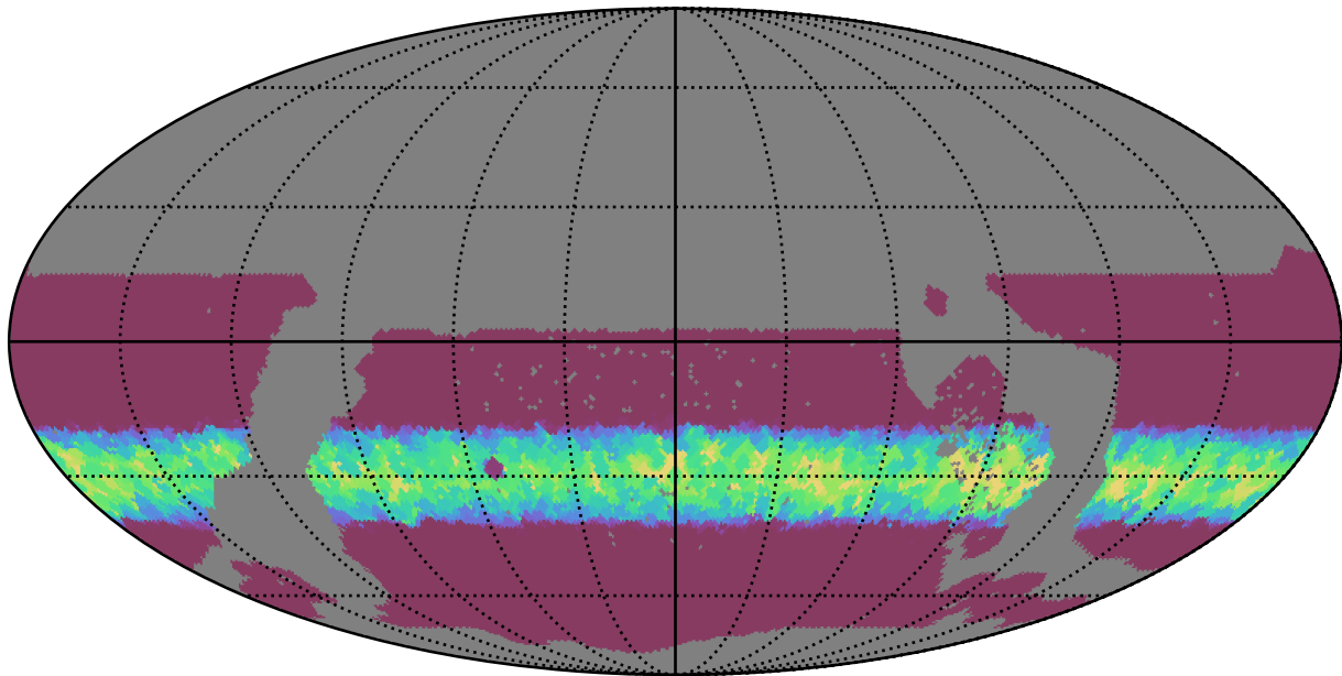
ddf_loaded_half_fl4_v3.4_10yrs WFD y band: Min normairmass
