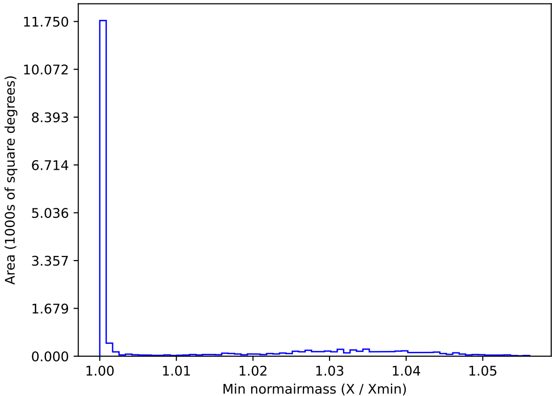
ddf_loaded_half_fl4_v3.4_10yrs WFD u band: Min normairmass
