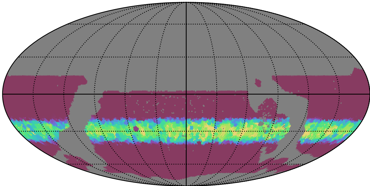
ddf_loaded_half_fl4_v3.4_10yrs WFD r band: Min normairmass
