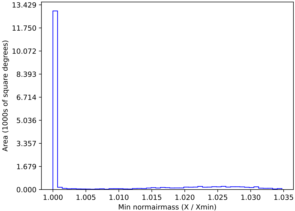
ddf_loaded_half_fl4_v3.4_10yrs WFD r band: Min normairmass
