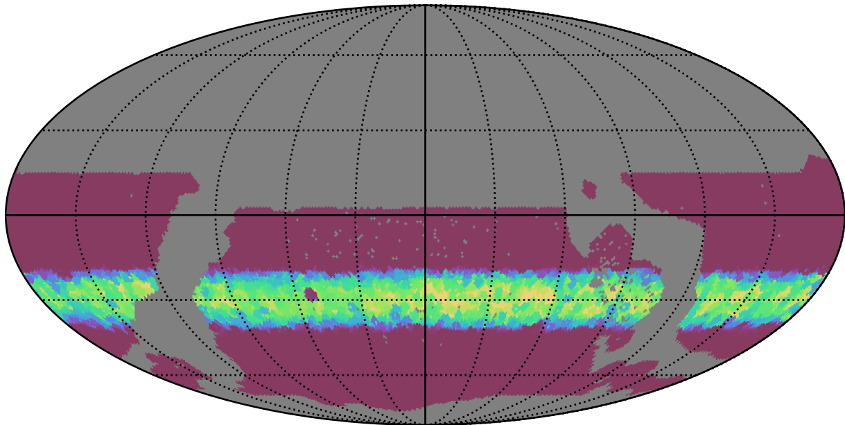
ddf_loaded_half_fl4_v3.4_10yrs WFD i band: Min normairmass
