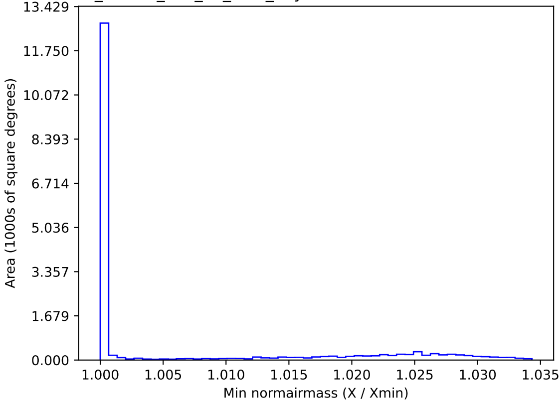
ddf_loaded_half_fl4_v3.4_10yrs WFD i band: Min normairmass
