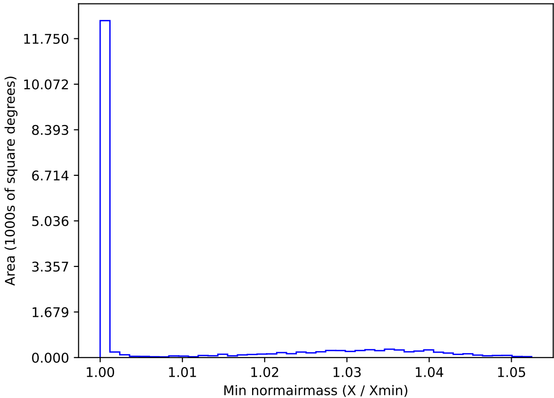
ddf_loaded_half_fl4_v3.4_10yrs WFD g band: Min normairmass
