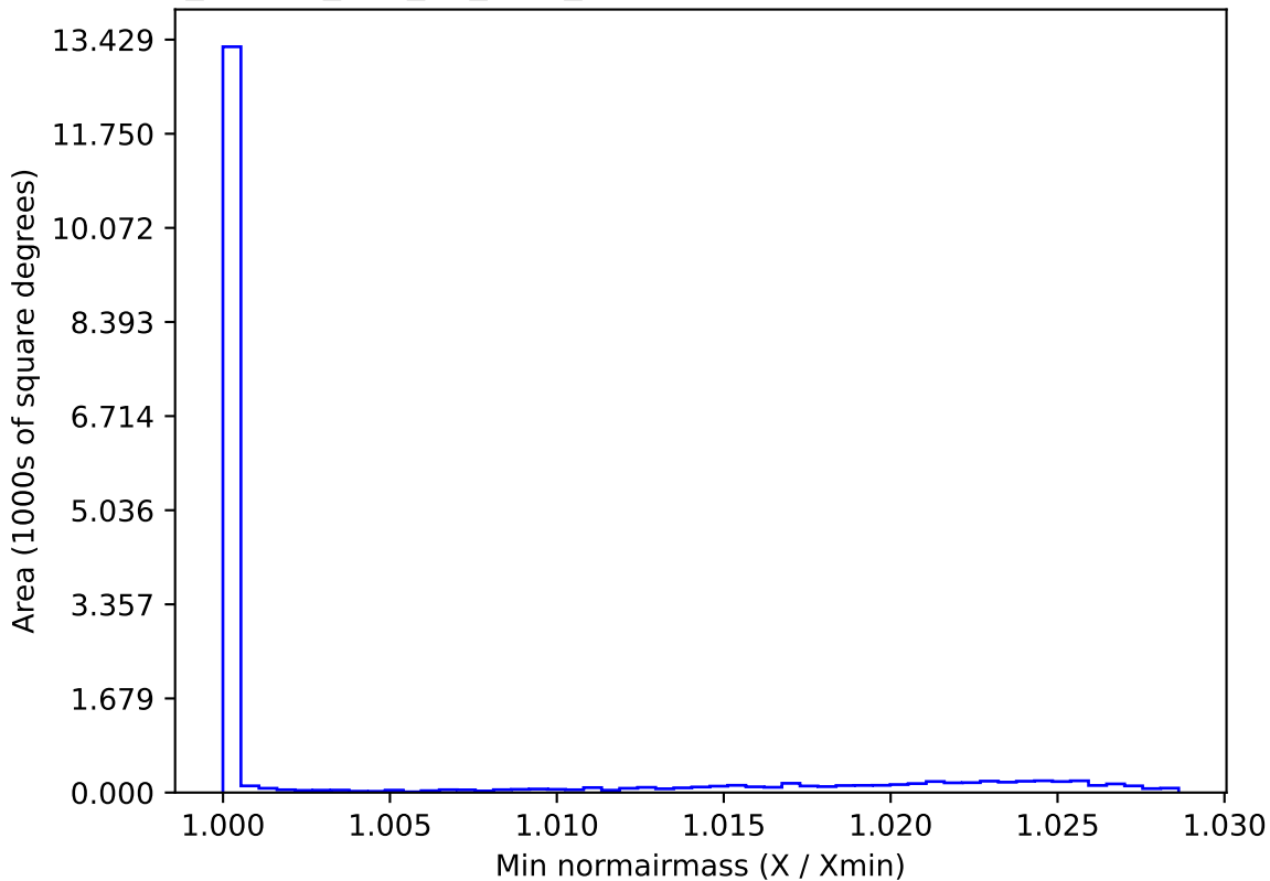
ddf_loaded_half_fl4_v3.4_10yrs WFD all bands: Min normairmass
