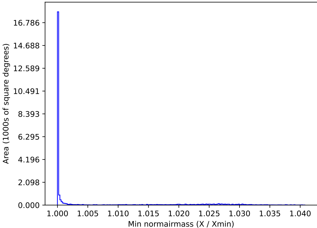
ddf_loaded_half_fl4_v3.4_10yrs All sky z band: Min normairmass
