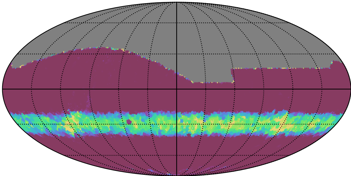
ddf_loaded_half_fl4_v3.4_10yrs All sky r band: Min normairmass
