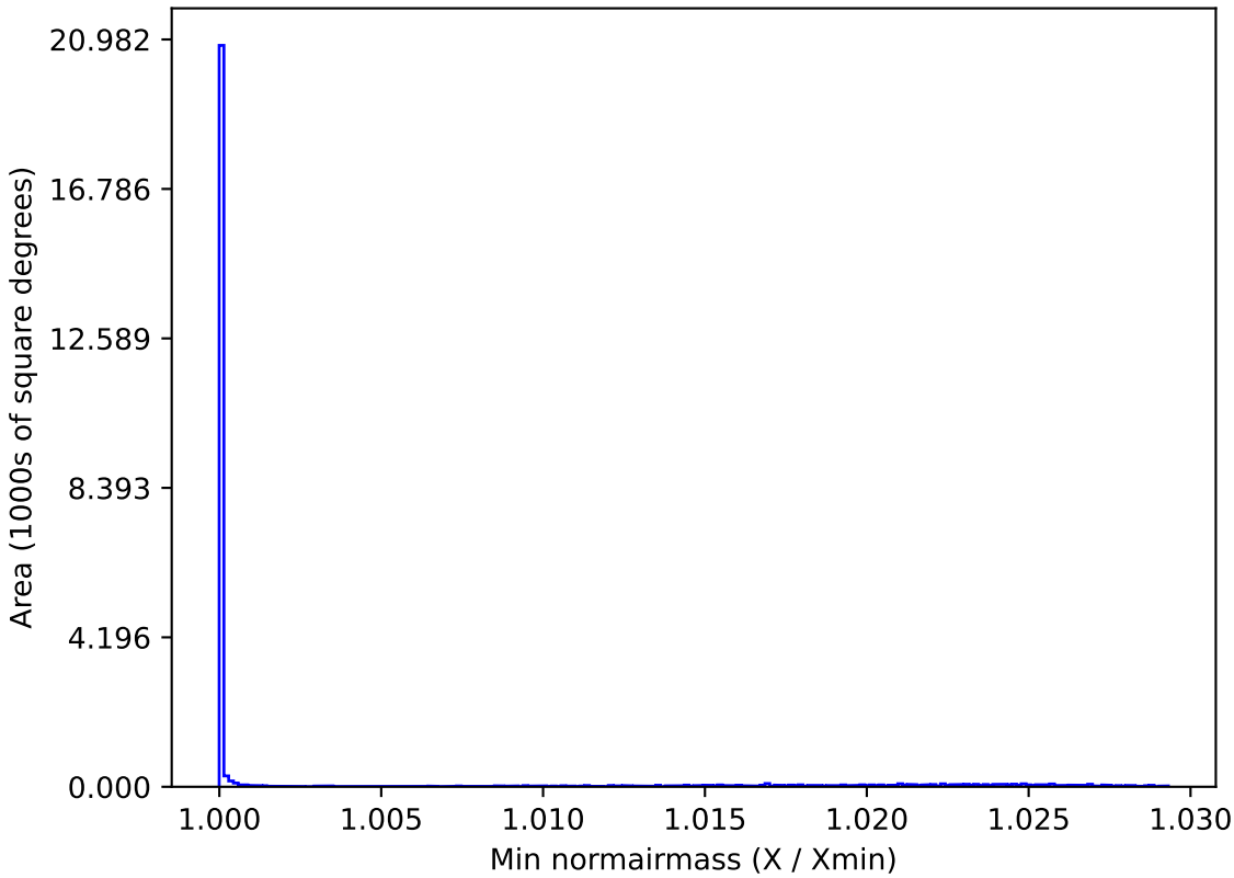
ddf_loaded_half_fl4_v3.4_10yrs All sky all bands: Min normairmass
