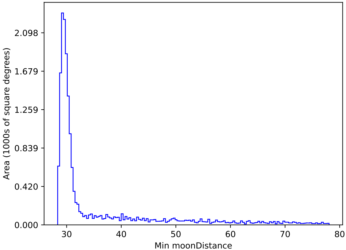
ddf_loaded_half_fl4_v3.4_10yrs WFD z band: Min moonDistance
