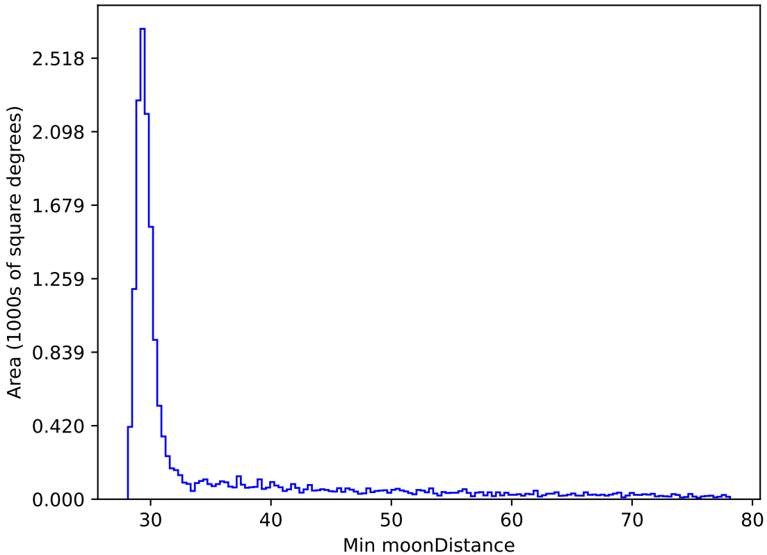
ddf_loaded_half_fl4_v3.4_10yrs WFD y band: Min moonDistance
