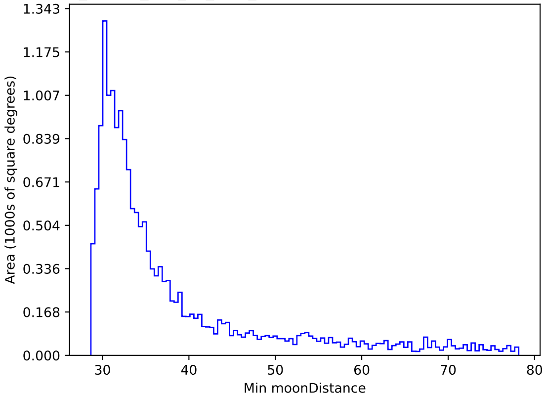
ddf_loaded_half_fl4_v3.4_10yrs WFD r band: Min moonDistance
