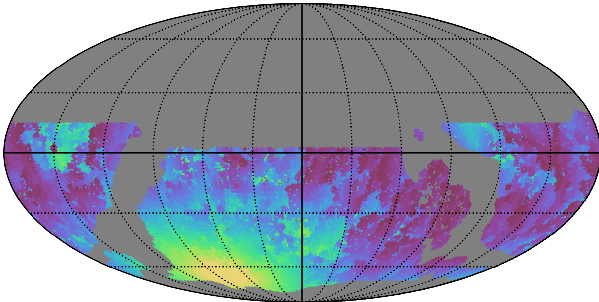
ddf_loaded_half_fl4_v3.4_10yrs WFD g band: Min moonDistance
