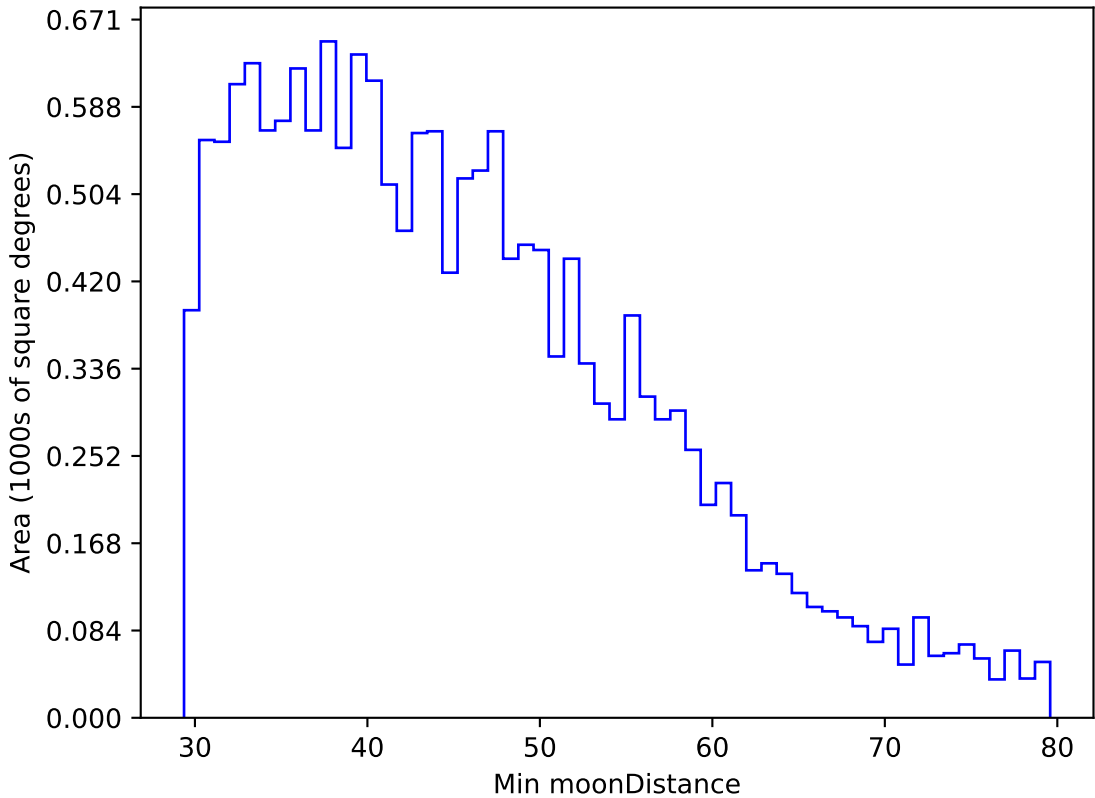
ddf_loaded_half_fl4_v3.4_10yrs WFD g band: Min moonDistance
