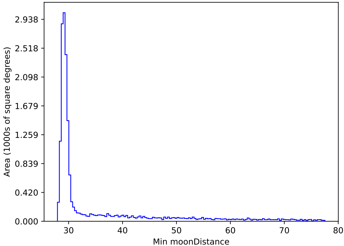
ddf_loaded_half_fl4_v3.4_10yrs WFD all bands: Min moonDistance
