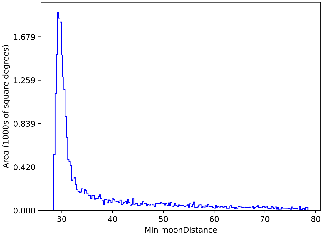
ddf_loaded_half_fl4_v3.4_10yrs All sky z band: Min moonDistance
