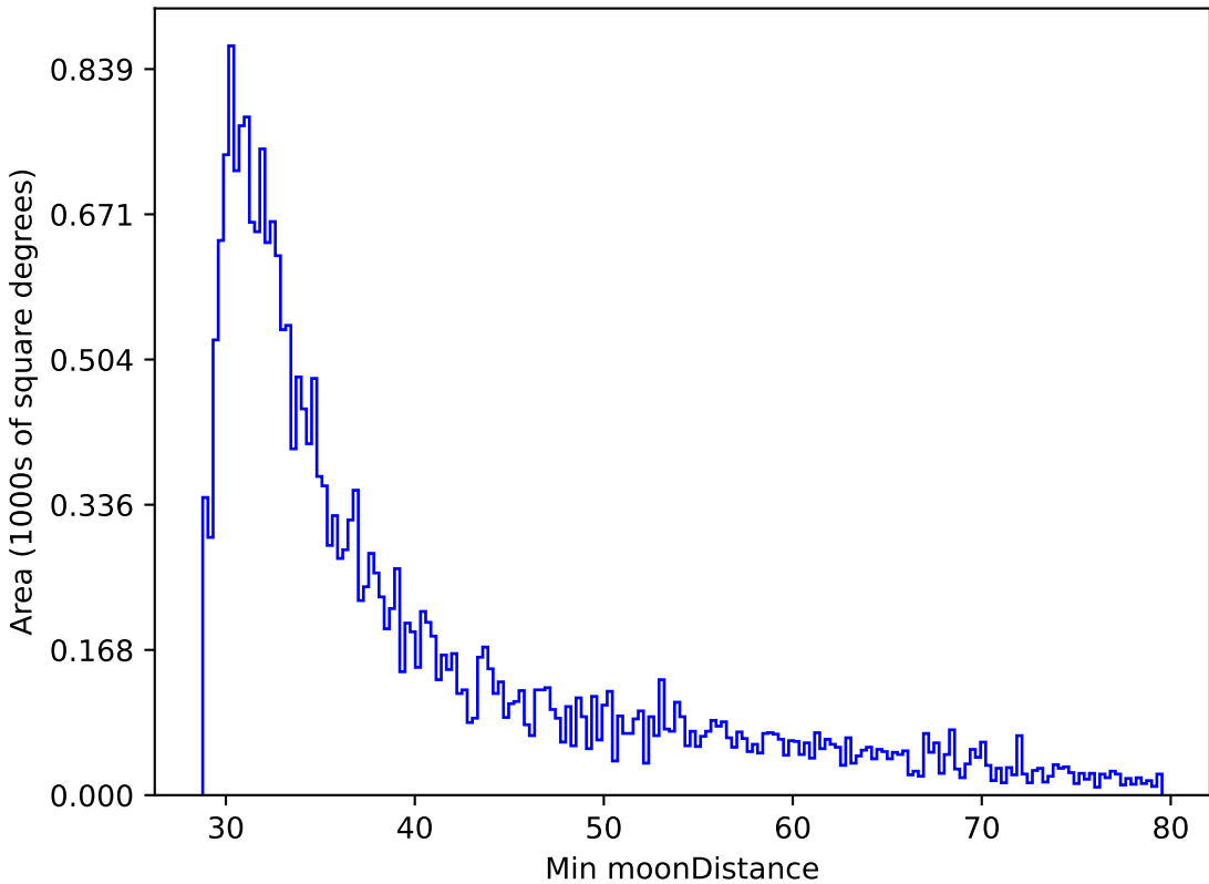
ddf_loaded_half_fl4_v3.4_10yrs All sky r band: Min moonDistance
