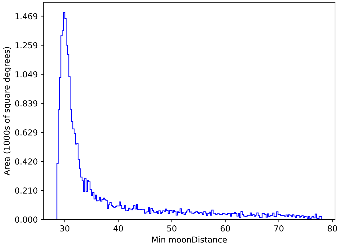
ddf_loaded_half_fl4_v3.4_10yrs All sky i band: Min moonDistance
