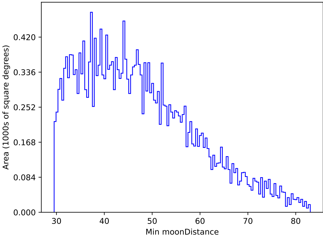
ddf_loaded_half_fl4_v3.4_10yrs All sky g band: Min moonDistance
